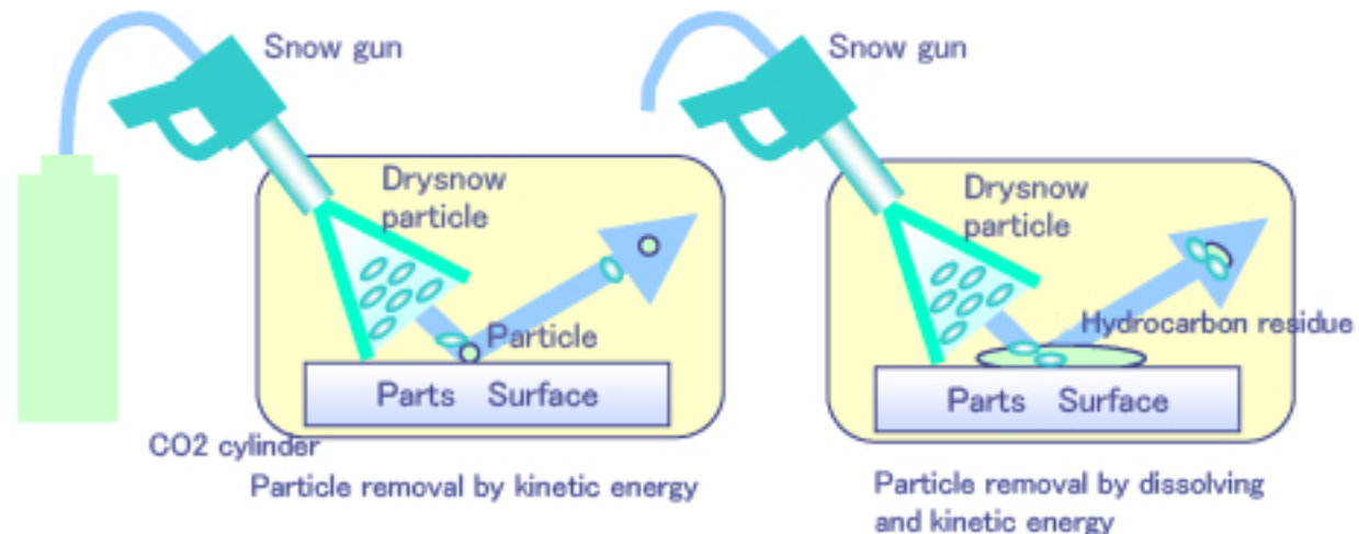
Drysnow injection state (Type DS-1)
